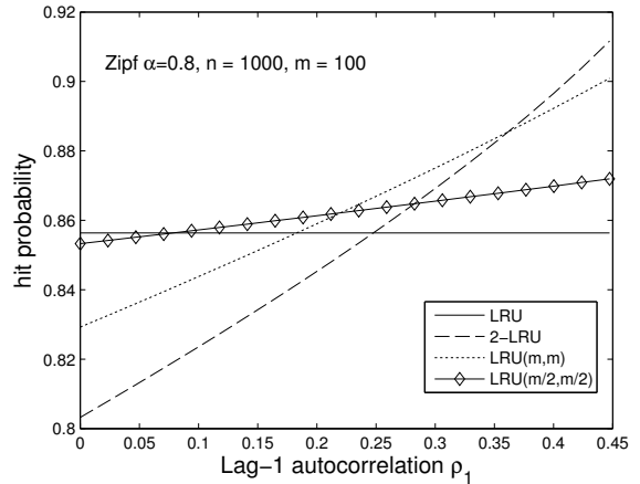
Fig. 4. Hit probability as a function of the lag-1 autocorrelation \rho_1 for LRU, \text{LRU}(m, m) , \text{LRU}(m/2, m/2) and 2-LRU when subject to MAP arrivals (with z = 10 ).
